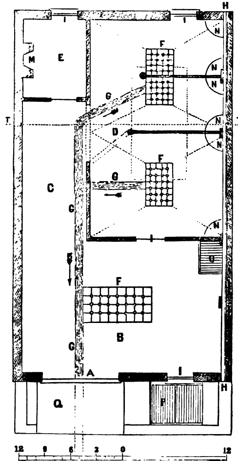
Ground Plan.
